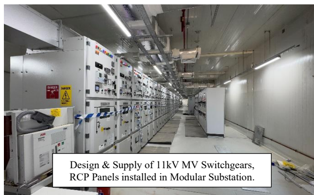
MV Panels
